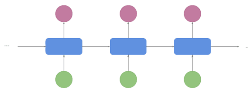
(4) N-N Tagging
