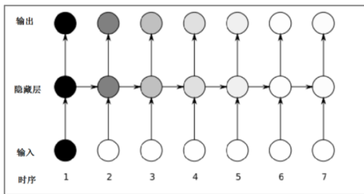
RNN
